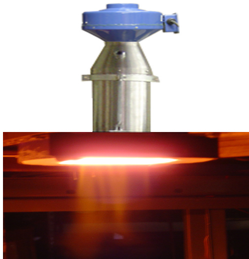
Exhibit 22: Plasma heating
