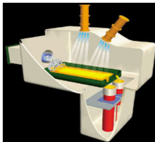
Exhibit 19: Electron Beam Cold-Hearth Refining
